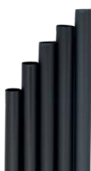
1CAN60 BOMBILLA RECTA NEGRAS BIO-ECO dimensioni size h 210mm / Ø 6mm pz/conf pcs/pack 150 pz/cart pcs/box 3450
